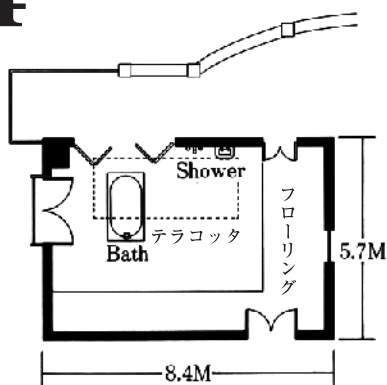
Room 4 : 8.4M × 5.7M × 3.2M. Bath & Shower
