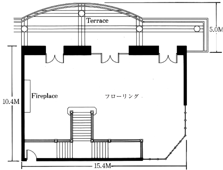
Room 1 : 15.4M × 10.4M × 5.0M. Fireplace & Terrace
