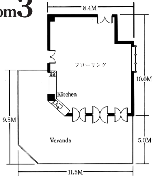
Room 3 : 10.0M × 8.4M × 3.6/3.2M. Kitchen & Veranda
